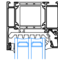
FIXED WINDOW
